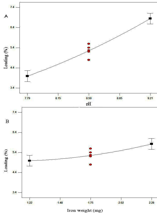
Fig 2. Main effects of pH (A) and iron weight (B) on IONPs loading (%) according to ANOVA table and obtained results. Main effects are significant on loading efficiency
