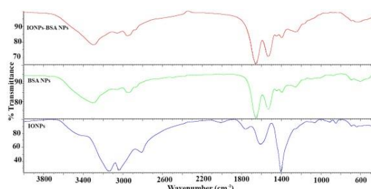
Fig 5. FTIR spectra of the IONPs (IONPs; blue), BSA NPs (BSA NPs; green) and IONPs-BSA NPs (IONPs-BSA NPs; red)
