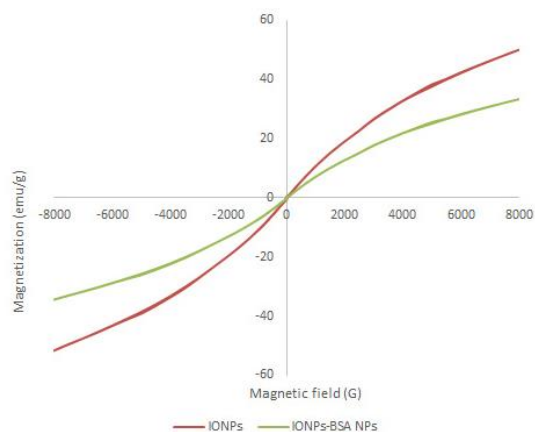
Fig 6. Magnetization curves of IONPs and IONPs-BSA nanoparticles
