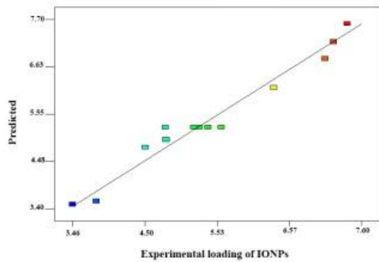
Fig 1. Predicted and actual IONPs loading efficiency (%) obtained from model simulation and experiments, respectively. Points are the actual amount of IONPs loading efficiency that approximately fit the model due to high amount of R^2 (0.96)
