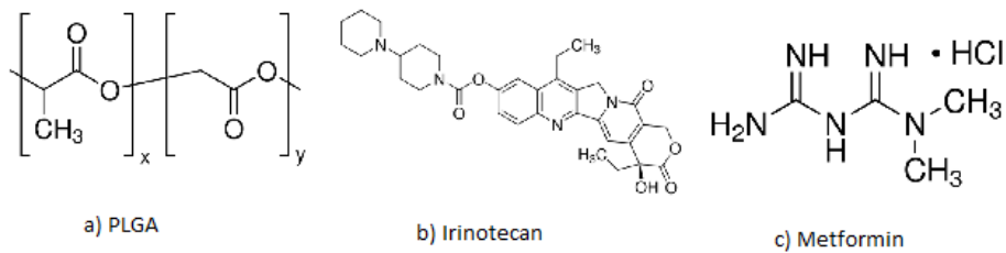
Fig 1. Chemicals structure of poly-D,L-lactide-co-glycolide, irinotecan and metformin
