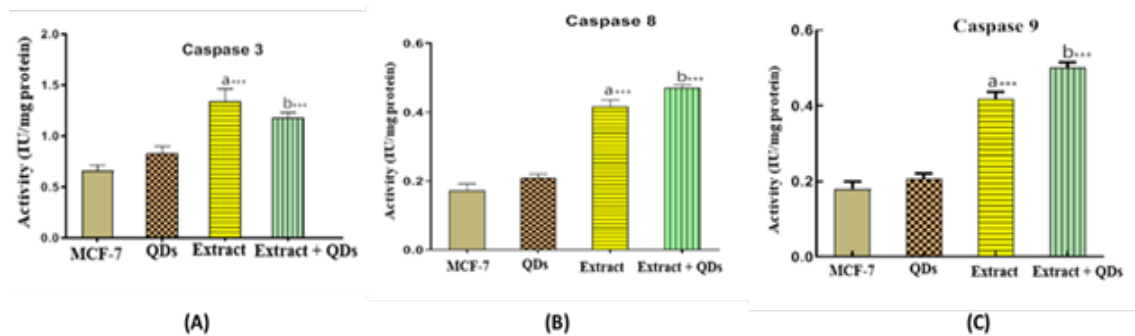
Fig. 4. The activity of caspases 3 (A), 8 (B) and 9 (C) in the studied groups.
