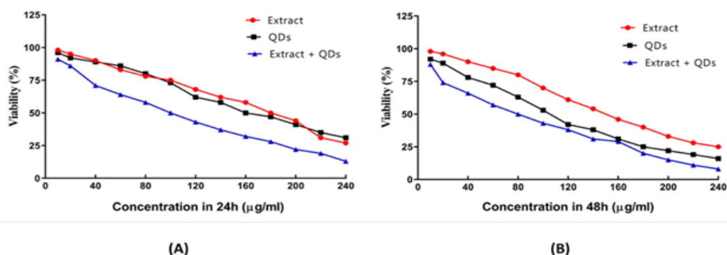
Fig. 2 Cytotoxic effect of different concentrations of N. oleander extract, CdTe QDs and N. oleander extract coated-CdTe QDs on the proliferation of MCF-7 in comparison with untreated cells (control) by MTT method After 24 (A) 48 (B) hours. Extract: Group treated with N. oleander , QDs: Group treated with CdTe QDs, Extract + QDs: Group treated with N. oleander -coated CdTe QDs. CdTe: cadmium telluride; N. oleander : Nerium oleander ; QD: quantum dots.
