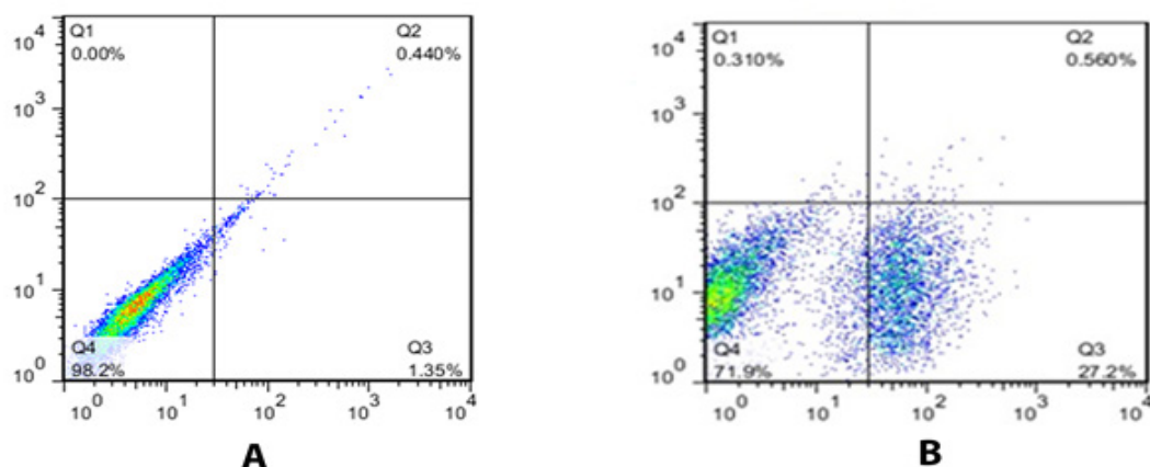
Fig 3. Apoptosis percentage in MCF7 cells after 24 h of treatment with N. oleander -coated CdTe QDs. A. Untreated group. B. Extract+QDs: Group treated with N. oleander -coated CdTe QDs. CdTe: cadmium telluride; N. oleander : Nerium oleander ; QDs: quantum dots.
