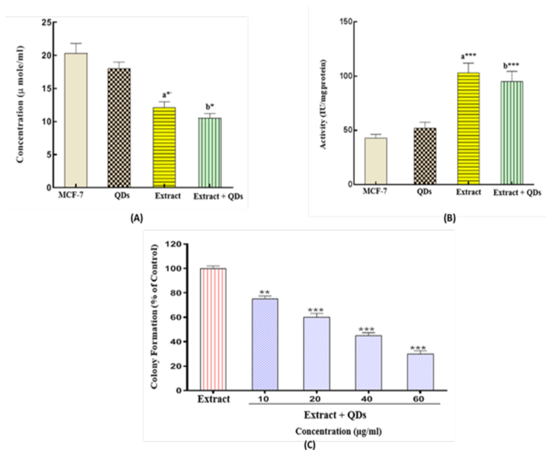
Fig. 6. Findings of measuring the amount of produced NO (A), alkaline phosphatase activity (B) and percentage of colony formation in the studied groups (C). Extract: Group treated with Nerium oleander , QDs: Group treated with CdTe QDs, Extract + QDs: Group treated with N. oleander -coated CdTe QDs. a: significant difference with MCF7 and QDs groups, b: significant difference with QDs group, ** :p < 0.01, *** :p < 0.001. CdTe: cadmium telluride; N. oleander : Nerium oleander ; QD: quantum dots.
