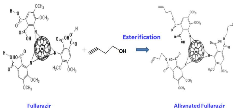
Fig. 2. Schematic of Alkynated Fullarazir
