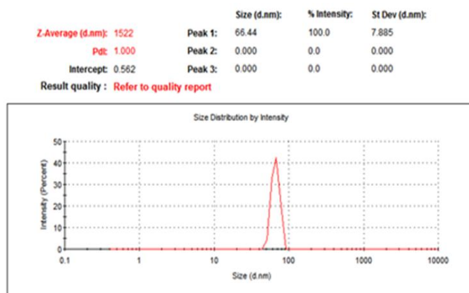
Fig. 7. Zeta size spectrum of NCDC
