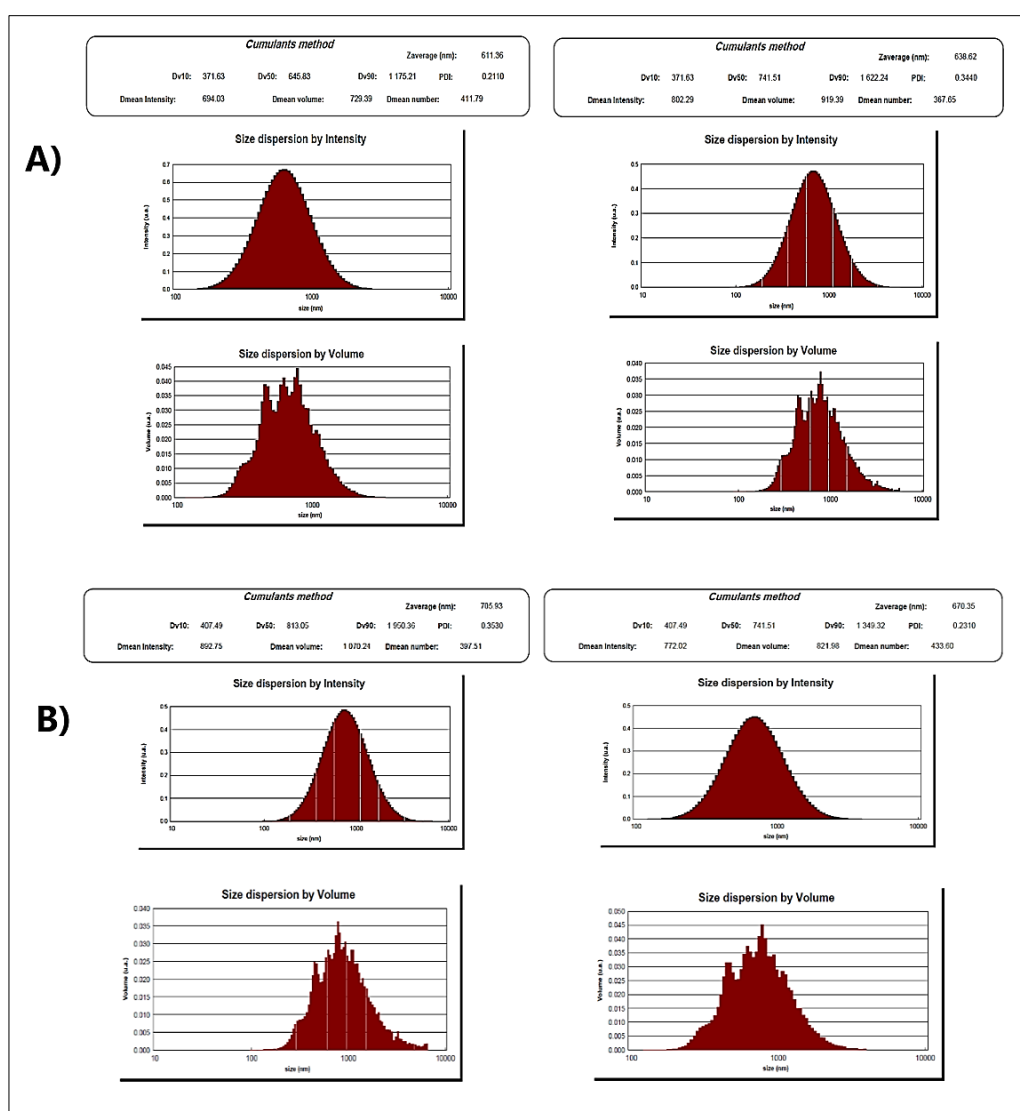
Fig. 2. Size of nanoparticles based on Dynamic Light Scattering (DLS) for A) \text{Fe}_3\text{O}_4 f-PEG-MET and B) \text{Fe}_3\text{O}_4 f-PEG-MET@MB. (MB: Methylene Blue, PEG: Polyethylene glycol, MET: Metformin)
