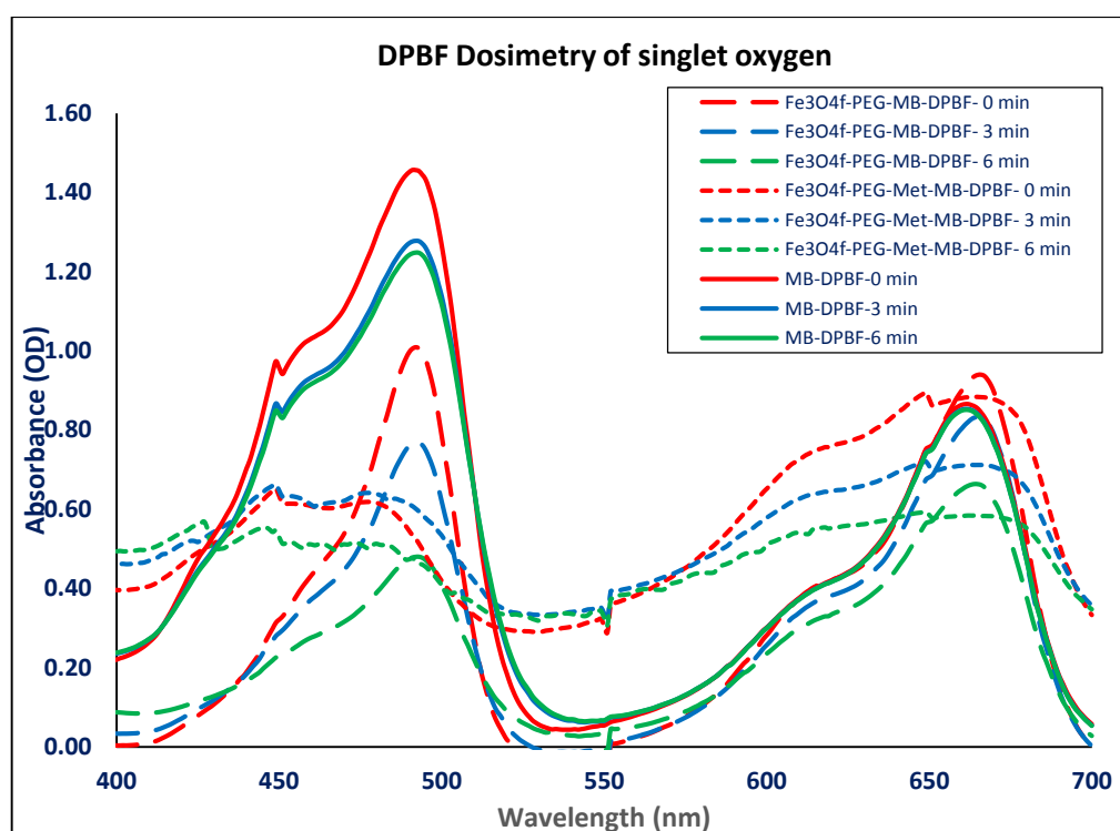
Fig. 13. DPBF dosimetry of ROS in different groups (Spectrophotometry analysis). ( MB : Methylene Blue, PEG : Polyethylene glycol, MET : Metformin). As it can be seen, \text{Fe}_3\text{O}_4\text{f-PEG-MB} structure is more efficient in DPBF photobleaching than free MB. This phenomenon can be caused by two reasons: 1) Prevention of methylene blue photobleaching during irradiation. 2) Preventing the dimerization of methylene blue by conjugating it inside the nanostructure. The DPBF curve in the presence of \text{Fe}_3\text{O}_4\text{f-PEG-MB-MET} caused changes in its spectrum shape, which could be due to the strong interaction between these two structures.
