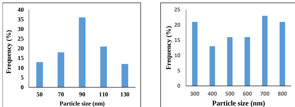
Fig. 5. Particle size distribution histogram of A) Fe 3 O 4 fluidic B) Fe 3 O 4 f-PEG-MET
