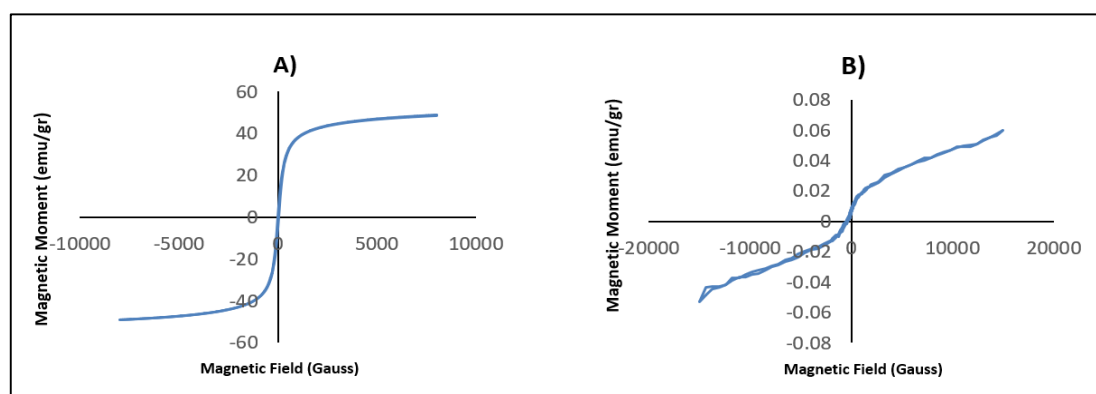
Fig. 11. The magnetization curve of A) ferrofluid or \text{Fe}_3\text{O}_4 , B) \text{Fe}_3\text{O}_4\text{f-PEG-MET} ( PEG : Polyethylene glycol, MET : Metformin)
