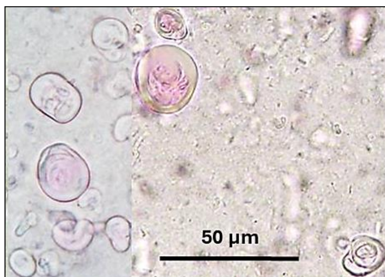
Fig. 6. Light microscopic images of silibinin and glycyrrhizic acid micrometric multilamellar vesicles
