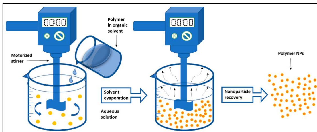
Fig. 2. Solvent-evaporation Technique [45]
