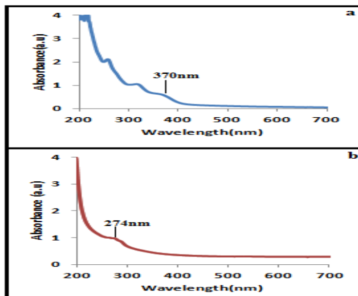
Fig. 1. UV-visible spectrum of chemical (a) and green synthesized (b) CuO-NPs
