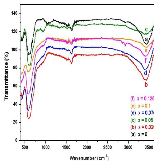
Figure 6. FTIR spectrums of the Zn_xFe_{3-x}O_4
