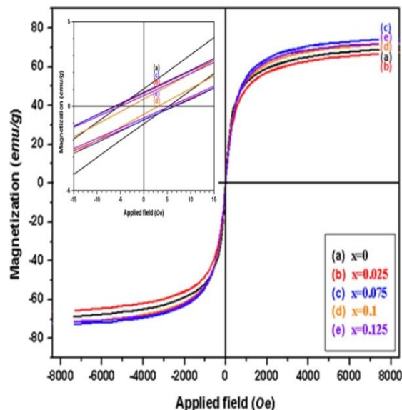
Figure 4. M-H curves of Zn x Fe 3-x O 4 nanoparticles with various Zn 2+ values in room temperature (The inset demonstrates the enlarged curves from -15 to 15 Oe).
